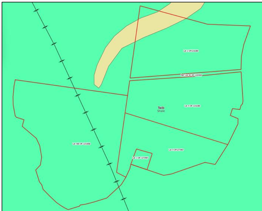
Figure 4: Penrith 1:100 000 Geological Sheet, for the revised ILP footprint. Coloured zones are pale green for 'Bringelly Shale' of the Wianamatta Group, and pale yellow for the fluvial sediments. The black line with convergent arrows indicates the mapped strike of the synclinal fold trough structure.
